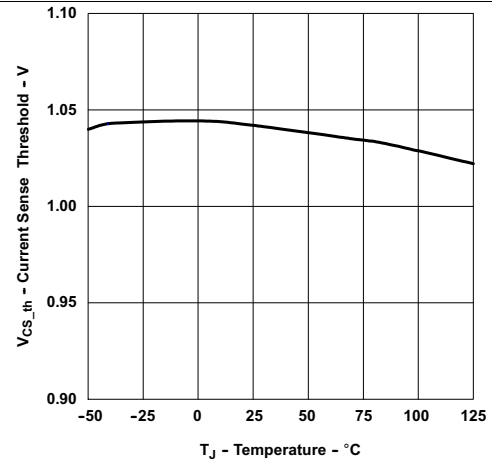
Figure 18. Current Sense Threshold Voltage vs Temperature
