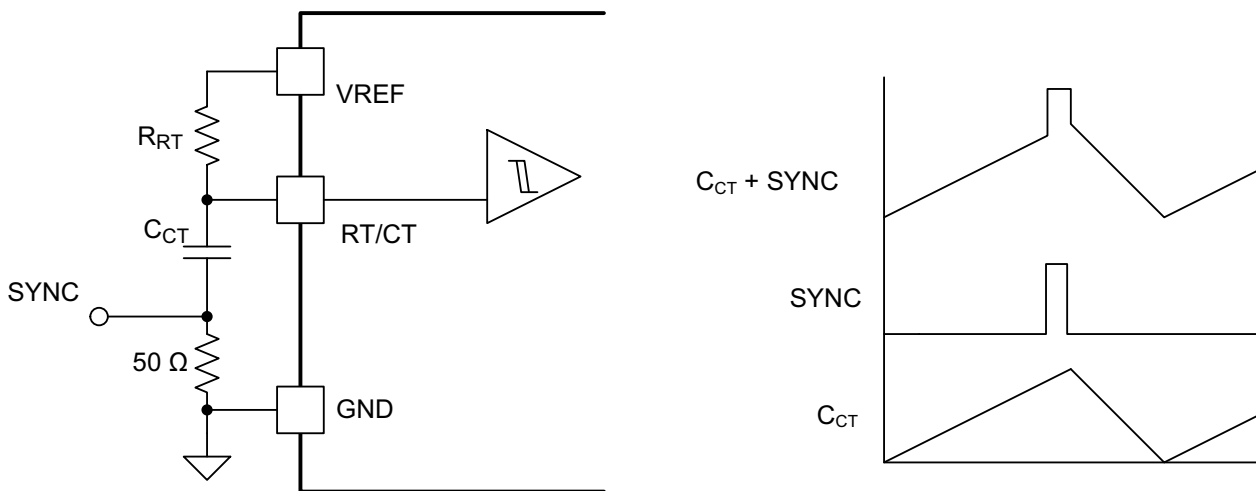
Figure 24. Oscillator Synchronization Circuit
