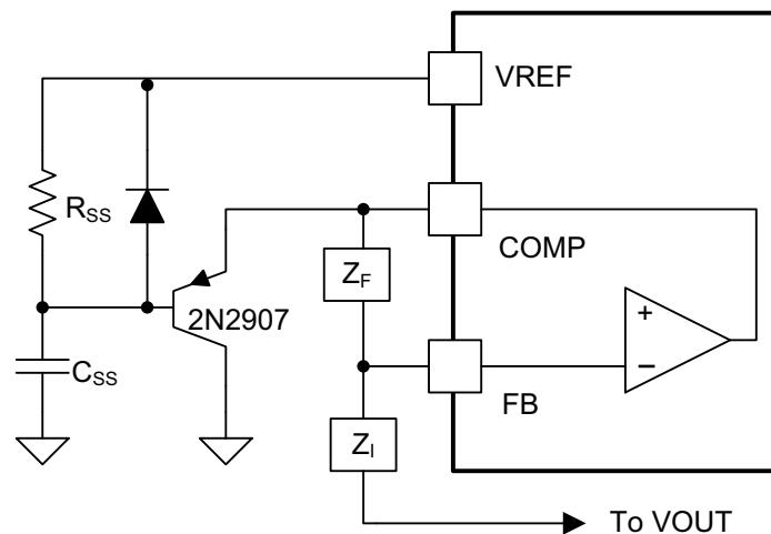
Figure 25. Soft-Start Implementation
