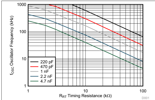
Figure 1. Oscillator Frequency vs Timing Resistance and Capacitance
