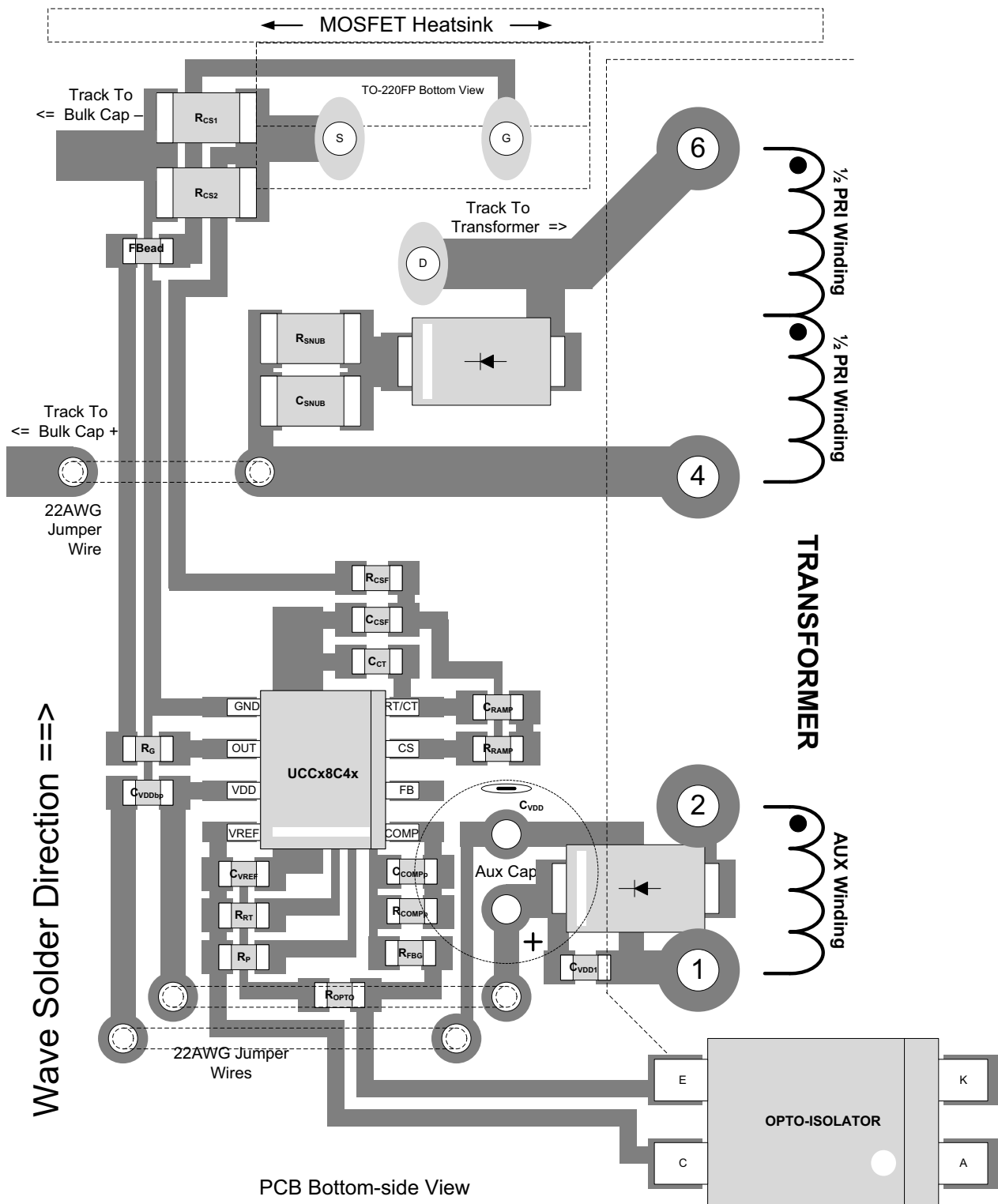
Figure 41. UCCx8C4x Layout Example
