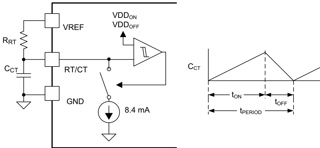
Figure 23. Oscillator Circuit
