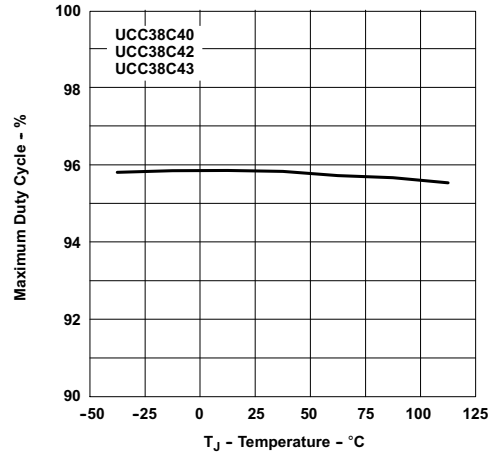
Figure 16. Maximum Duty Cycle vs Temperature
