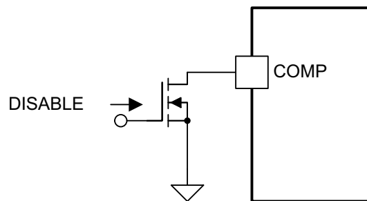
Figure 26. Disable Circuit
