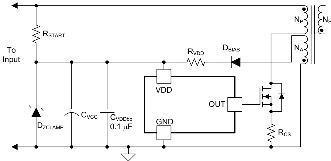
Figure 20. VDD Protection
