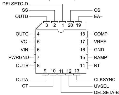
PLCC-20 Q PACKAGE (TOP VIEW)
