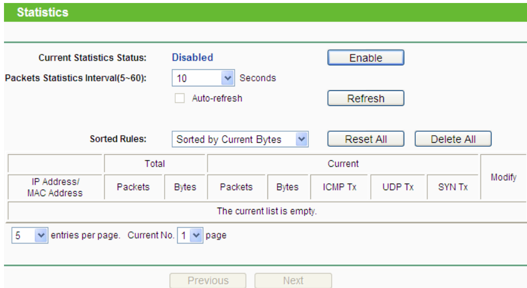
Figure 4-41 Statistics
