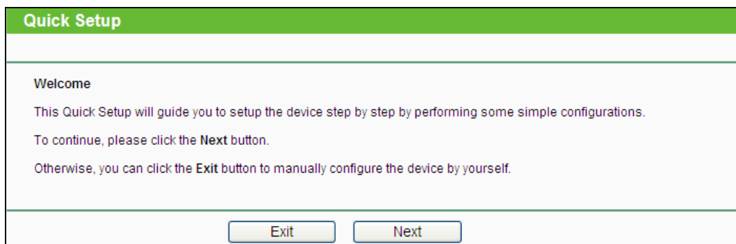
Figure 3-3 Quick Setup
