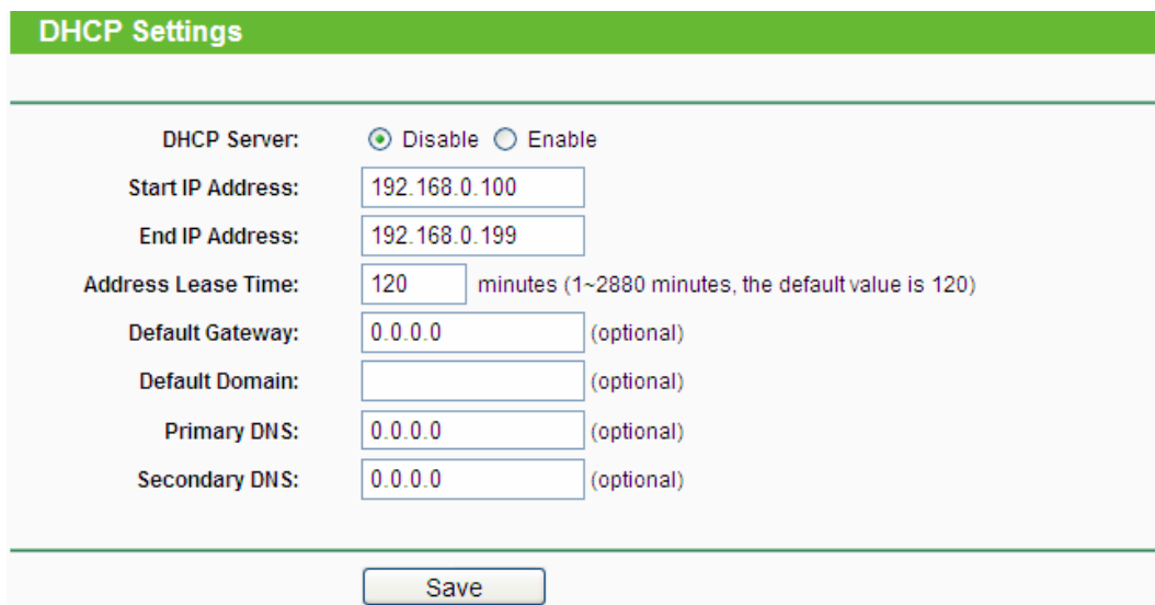
Figure 4-27 DHCP Settings
