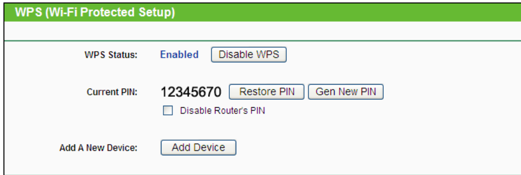
Figure 4-5 WPS
