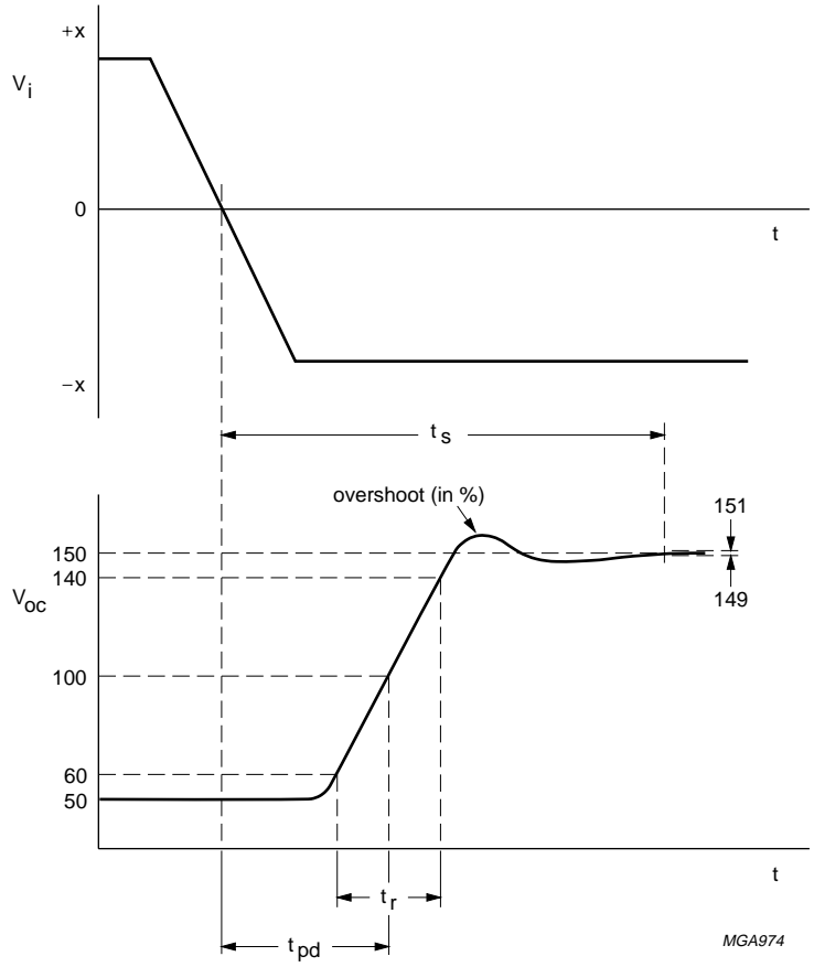
Fig.4 Output voltage (pin 8) rising edge as a function of the AC input signal.
