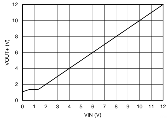
Figure 6. Positive Output Voltage Node vs Input Voltage
