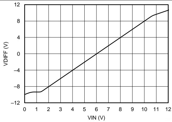
Figure 5. Differential Output Voltage vs Input Voltage
