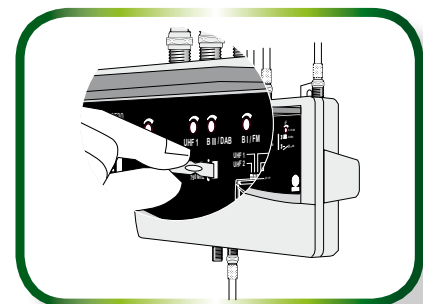
Switchable frequency range by inserting a plug-in bridge supplied
