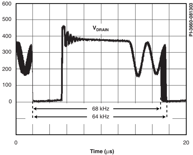
Figure 4. Frequency Jitter.
