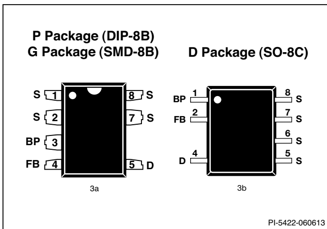
Figure 3. Pin Configuration.
