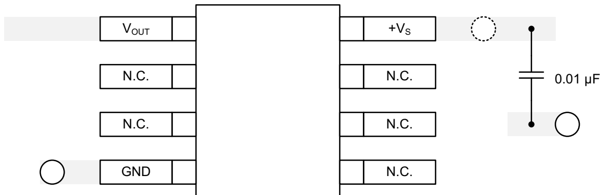
Figure 28. Layout Example
