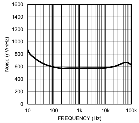
Figure 10. Noise Voltage
