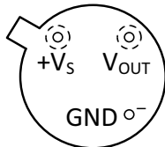
NDV Package 3-Pin TO-CAN (Bottom View)
