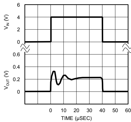
Figure 11. Start-Up Response
