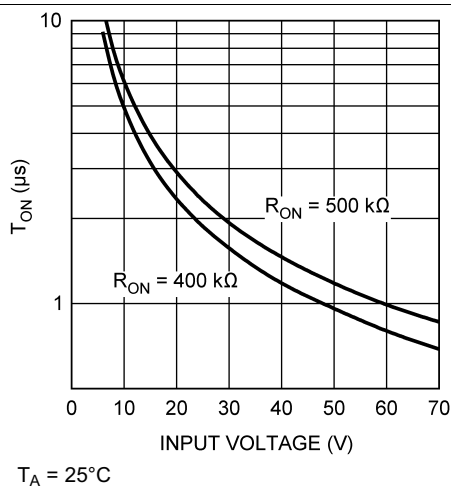
Figure 9. T_{ON} vs V_{IN}
