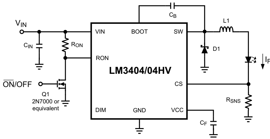
Figure 19. Low-Power Shutdown
