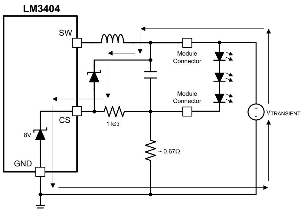
Figure 23. CS Pin With OVP, Transient Path
