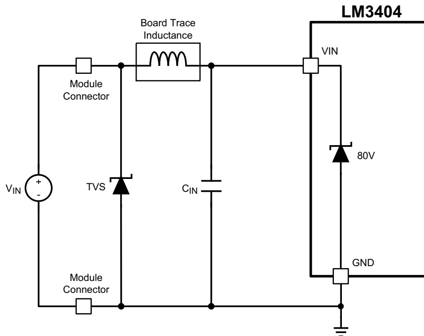
Figure 25. VIN Pin With Typical Input Protection
