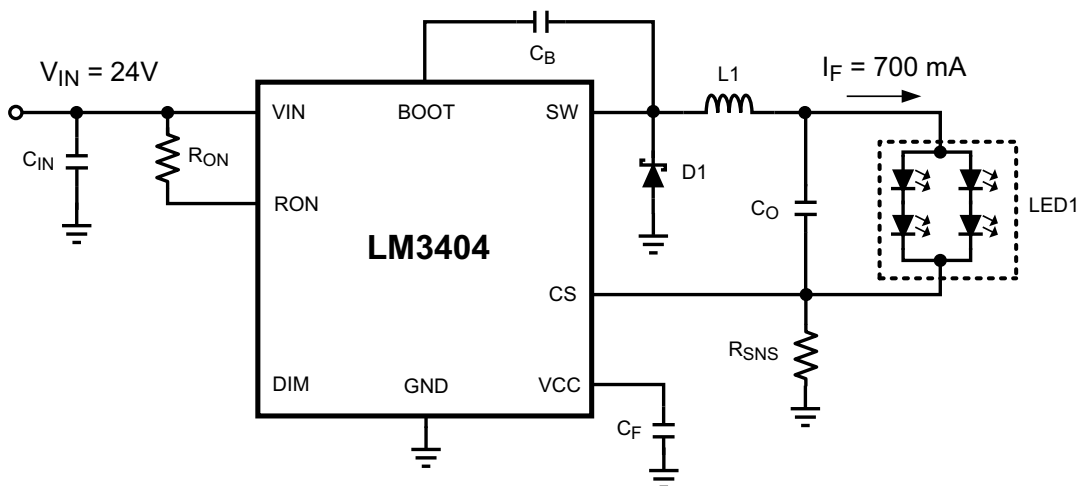
Figure 27. Schematic for Design Example 1
