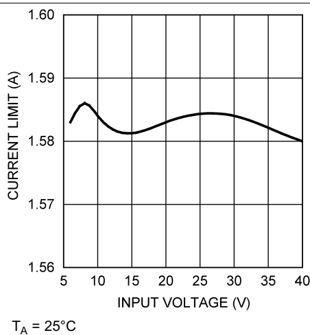
Figure 5. Current Limit vs V_{IN} , LM3404
