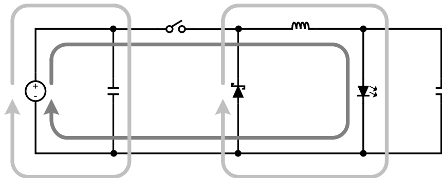
Figure 33. Buck Converter Current Loops
