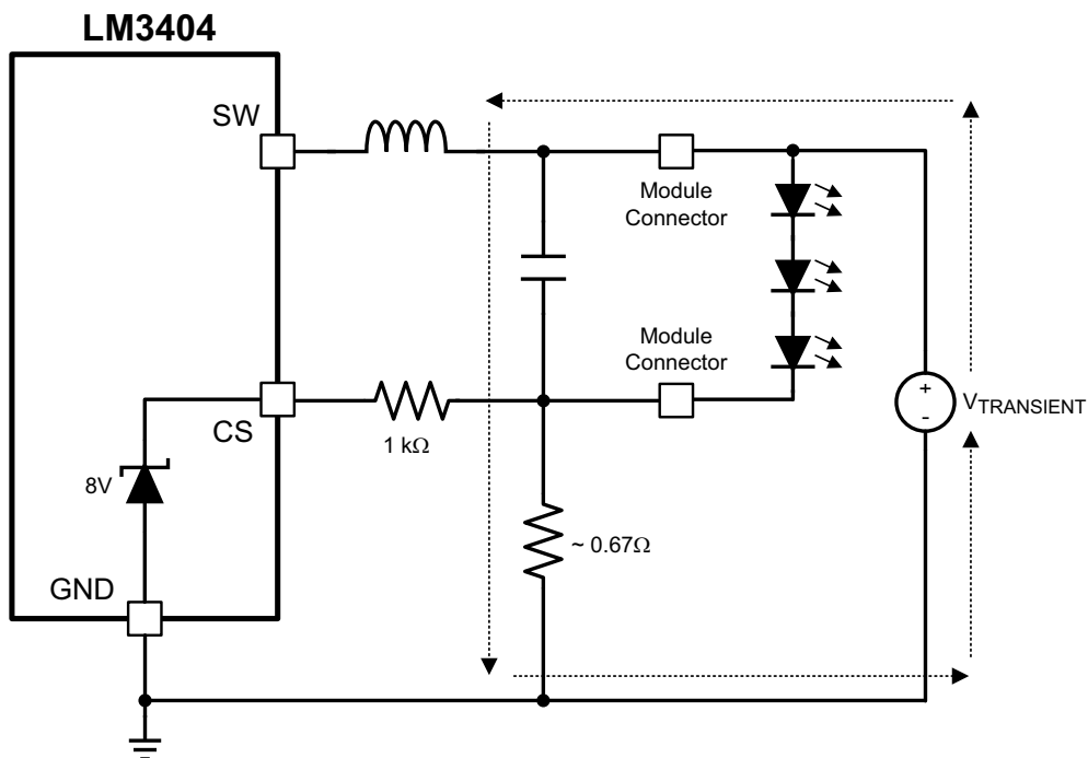
Figure 22. CS Pin, Transient Path With Protection
