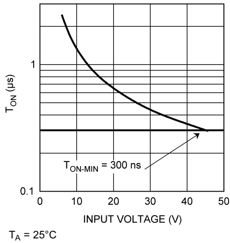
Figure 7. T_{ON} vs V_{IN} , R_{ON} = 100 k \Omega
