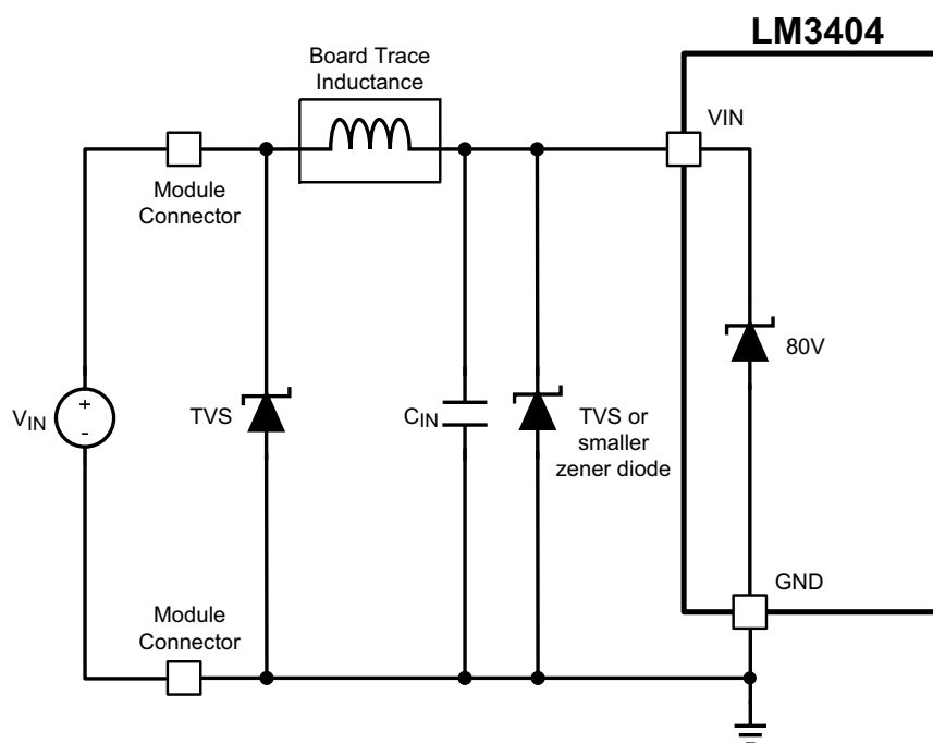
Figure 26. VIN Pin With Additional Input Protection
