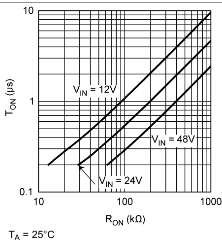
Figure 11. T_{ON} vs R_{ON} , LM3404HV
