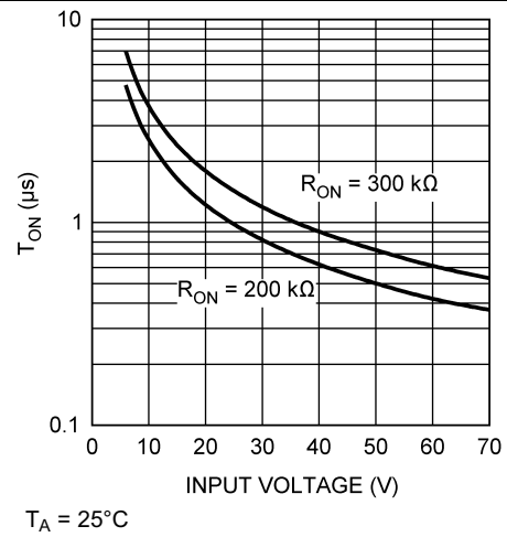
Figure 8. T_{ON} vs V_{IN}
