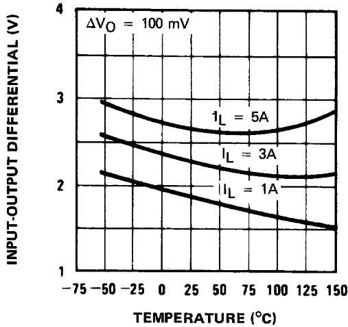
TEMPERATURE STABILITY
