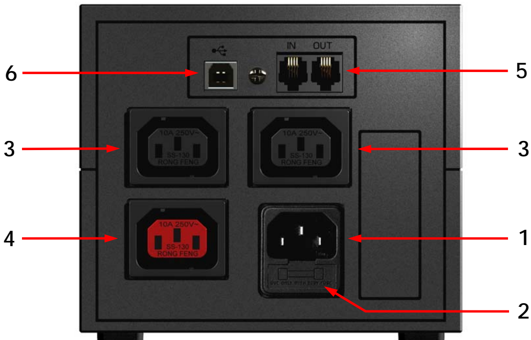
Figure 2 - Rear Side
