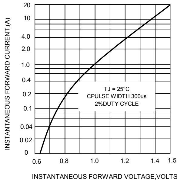
FIG.2-TYPICAL FORWARD CHARACTERISTICS
