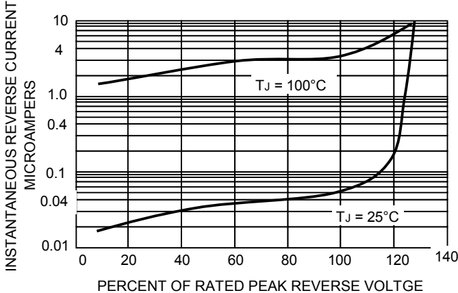
FIG.6-TYPICAL REVERSE CHARACTERISTICS
