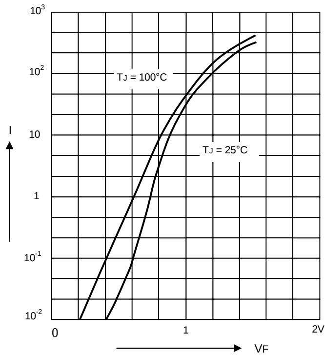
FIG.2-FORWARD CHARACTERISTICS
