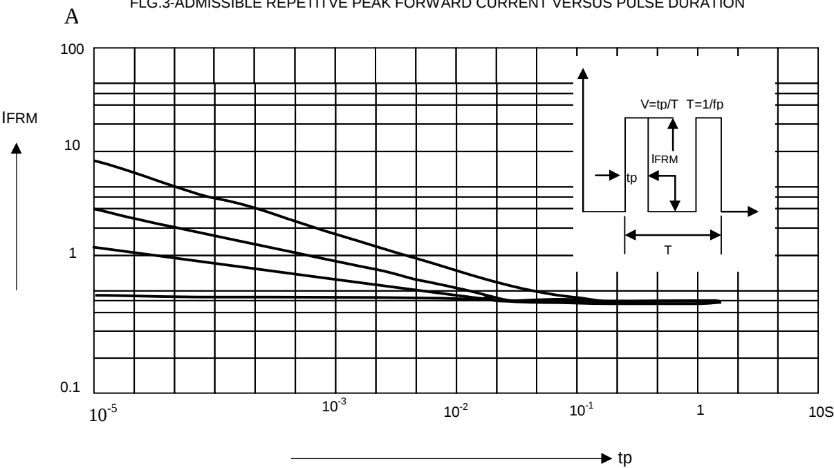
FIG.3-ADMISSIBLE REPETITIVE PEAK FORWARD CURRENT VERSUS PULSE DURATION
