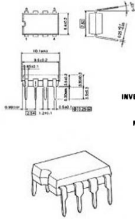
Dual-In-Line/SOIC Package
