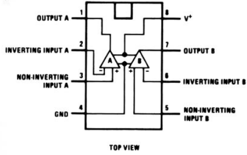
Dual-In-Line/SOIC Package
